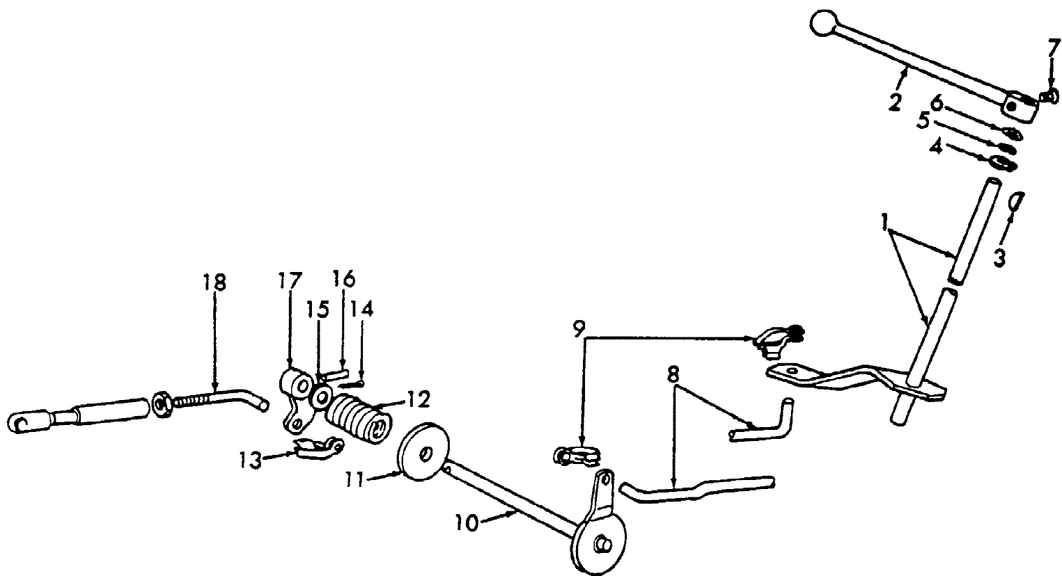
THROTTLE CONTROL PNEUMATIC GOVERNOR
