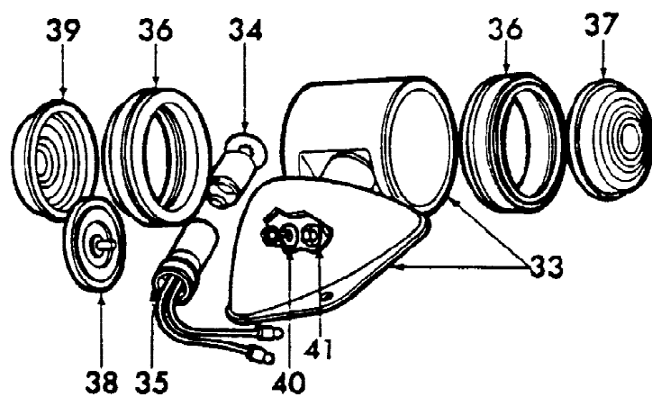
SIDE AND REAR LAMPS
