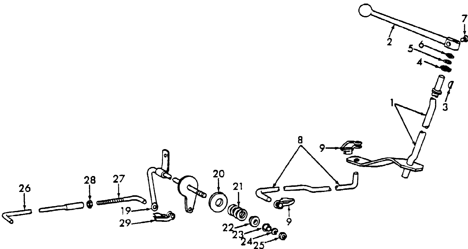
THROTTLE CONTROL MECHANICAL GOVERNOR
